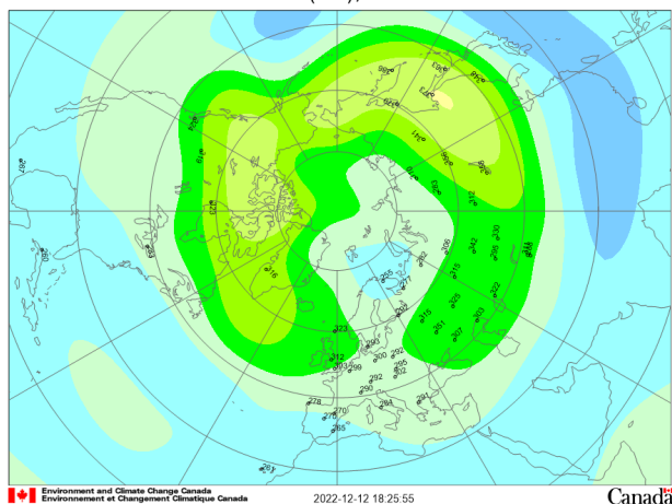
Mean total ozone (DU), 2022/11/01-2022/11/30
