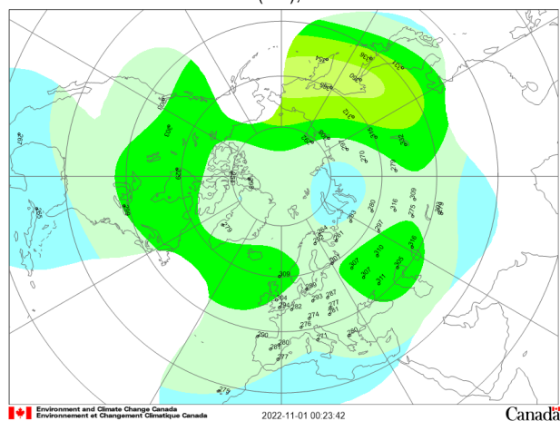
Mean total ozone (DU), 2022/10/01-2022/10/31
